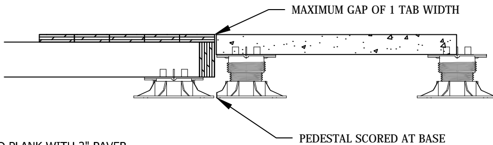
JOIST AND PLANK WITH 2" PAVER
