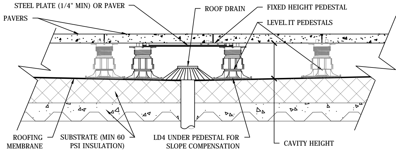
A1 DRAIN PEDESTAL PLACEMENT SECTION DETAIL
