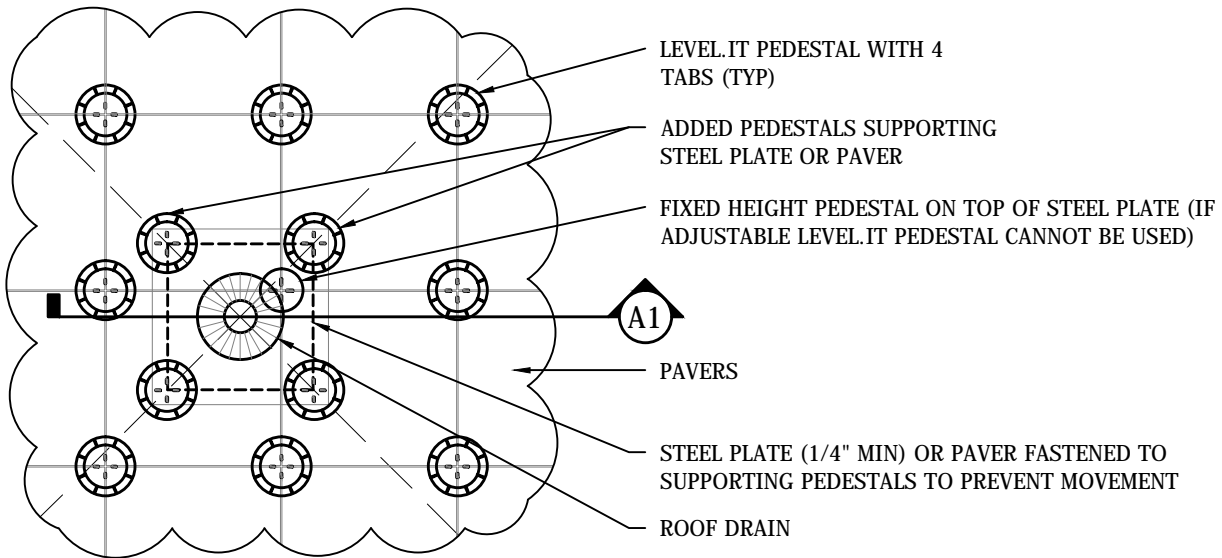
ENLARGED PLAN VIEW
