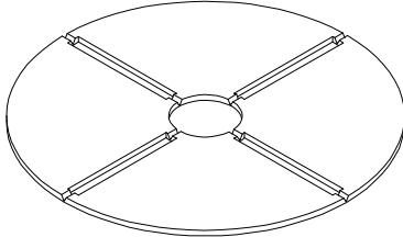
B11 1/16" FLEXIBLE SHIM 5 7/8" DIAMETER USED FOR SOUND DAMPENING AND FINAL SHIM LEVELING
